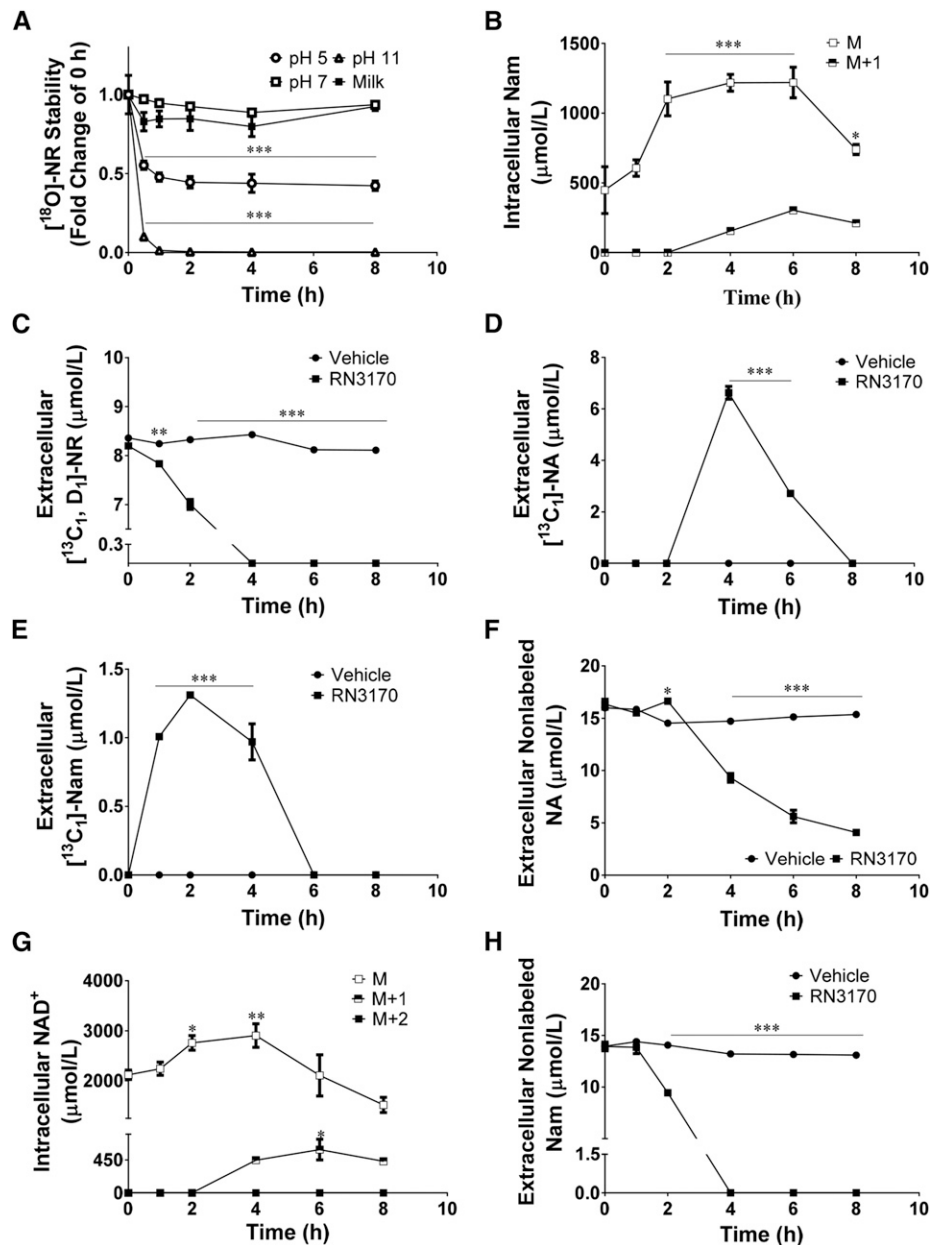
FIGURE 1 NR is stable in milk and is degraded by S. aureus . (A) Stability of [ ^{18}\text{O} ]-NR in 4 store-bought brands of skim milk and in water at pH 5, 7, and 11 ( n = 3 ) was assessed with LC-MS/MS. NR metabolism by S. aureus was determined with [ ^{13}\text{C}_1 , \text{D}_1 ]-NR and LC-MS (B–H). (B–F) Extracellular concentration of [ ^{13}\text{C}_1 , \text{D}_1 ]-NR, nonlabeled Nam, [ ^{13}\text{C}_1 ]-Nam, nonlabeled NA, and [ ^{13}\text{C}_1 ]-NA in Todd-Hewitt + 50 mmol/L Bis-Tris (pH 6.7) media containing 10 \mu\text{mol/L} [ ^{13}\text{C}_1 , \text{D}_1 ]-NR incubated at 37°C without or with S. aureus RN3170 inoculation ( n = 3 for inoculated media). In each panel, the concentration of the metabolite is shown in the noninoculated media ( n = 1 ). (G) Intracellular concentration of endogenous or ^{13}\text{C}_1 enriched Nam. (H) Intracellular concentration of endogenous ^{13}\text{C}_1 - or ^{13}\text{C}_1 , \text{D}_1 -enriched \text{NAD}^+ from extracts of S. aureus RN3170 cell pellets ( n = 3 /time point). For intracellular measurements, a Holm-Sidak multiple-comparisons post hoc test was performed to test for statistical significance compared with time point zero for each metabolite (B and G). For extracellular measurements, a Holm-Sidak multiple-comparisons test was performed to test for statistical significance compared with noninoculated medium within each time point (C–F and H). Data are represented as means \pm SEMs. * P < 0.05 , ** P < 0.01 , and *** P < 0.001 . NA, nicotinic acid; Nam, nicotinamide; NR, nicotinamide riboside.
